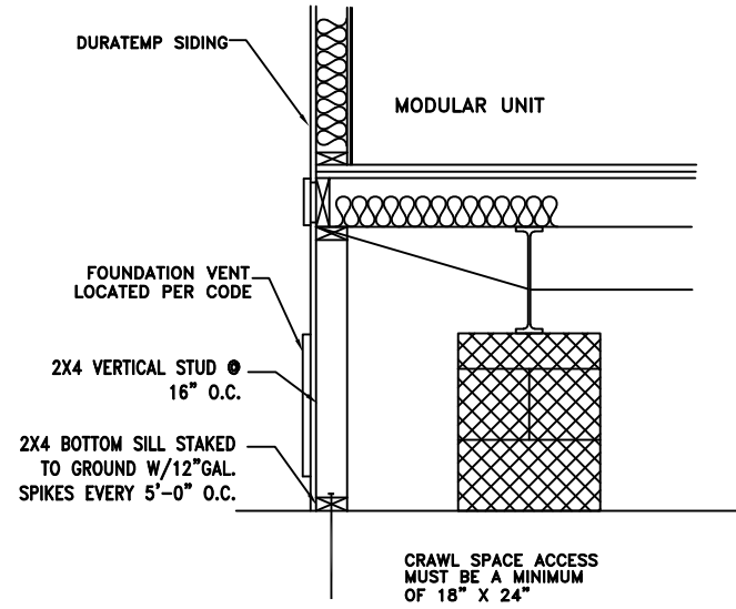
OUTRIGGER SKIRTING DETAIL
