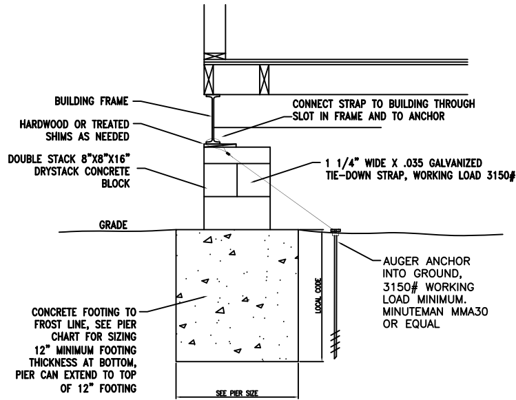
PIER DETAIL @ CORNER
